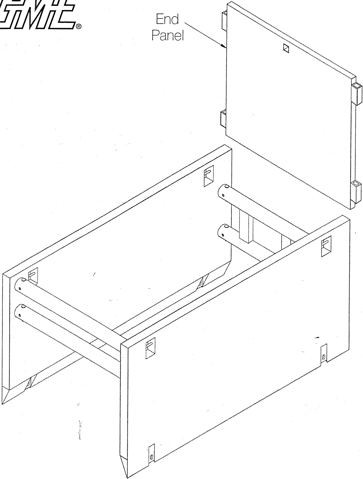
End Panel Configuration
